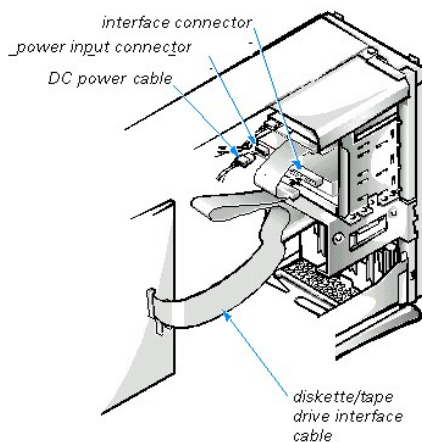
Figure 9. Attaching Diskette Drive or Tape Drive Cables
