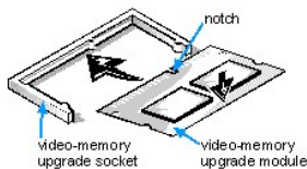
Figure 9. Installing a Video-Memory Upgrade Module
