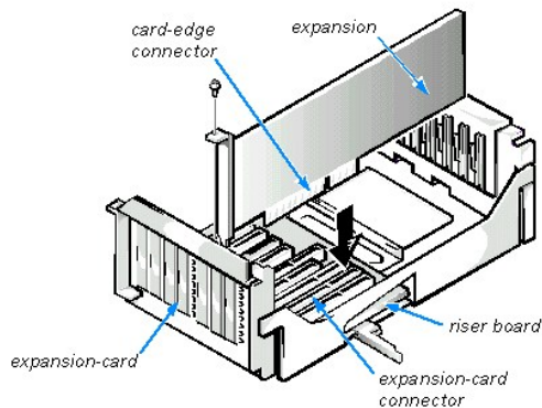
Figure 5. Installing an Expansion Card
