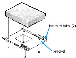
Figure 7. Attaching the Drive Bracket to the New Drive
