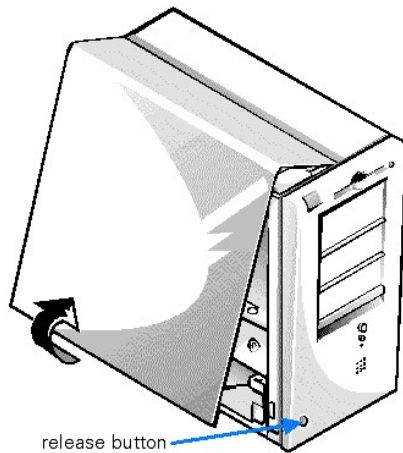
Figure 2. Removing the Computer Cover
