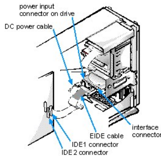
Figure 13. Attaching Hard-Disk Drive Cables
