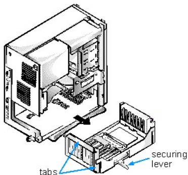
Figure 7. Removing the Expansion-Card Cage
