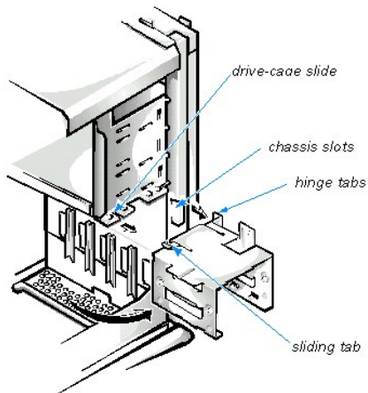
Figure 10. Removing the Hard-Disk Drive Bracket
