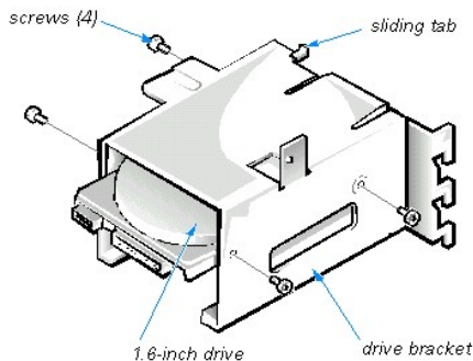
Figure 11. Inserting a 1.6-Inch Hard-Disk Drive in the Bracket
