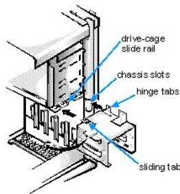
Figure 12. Inserting the Drive Bracket in the Chassis
