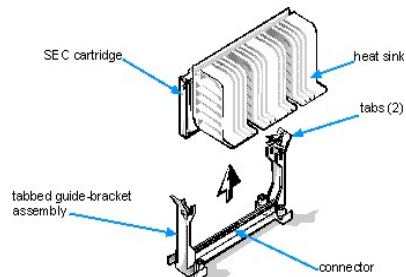
Figure 10. Removing the Microprocessor
