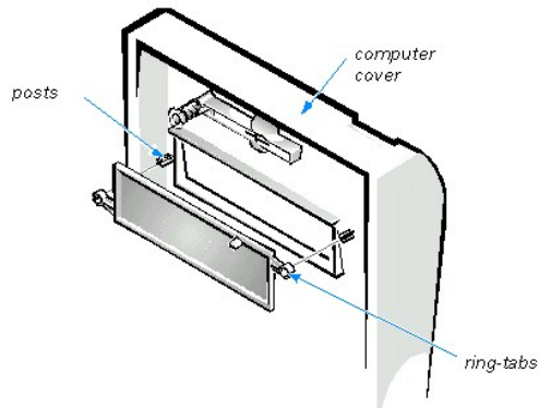
Figure 3. Removing the Front-Panel Insert for a 5.25-Inch Bay
