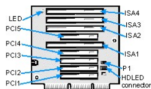
Figure 3. Riser-Board Expansion-Card Connectors
