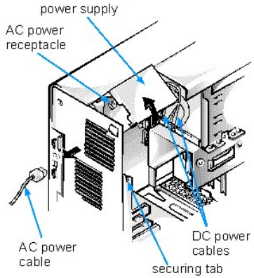
Figure 8. Rotating the Power Supply
