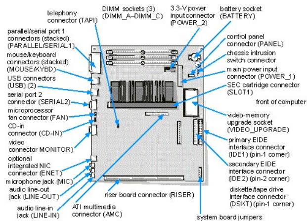
Figure 1. System Board Features
